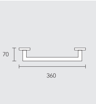
Handgreep
