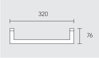
Handgreep
