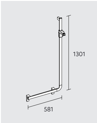
Angle bar 90° Hand shower sliding rail, right-hand model
