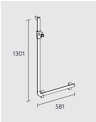
Angle bar 90° Hand shower sliding rail, left-hand model
