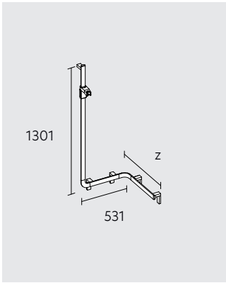
Rail system left-hand model
