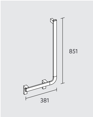
Angle bar 90° right-hand model
